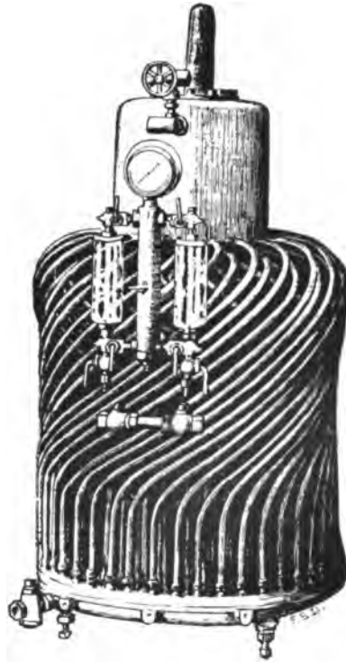
FIG. 170.—The "Lifu" Steam Boiler, showing arrangement and inclination of the tubes. The central steam drum terminates in two legs at the bottom, which are connected at either side to the annular mud-and-water drum at the base, thus completing the circulation.
